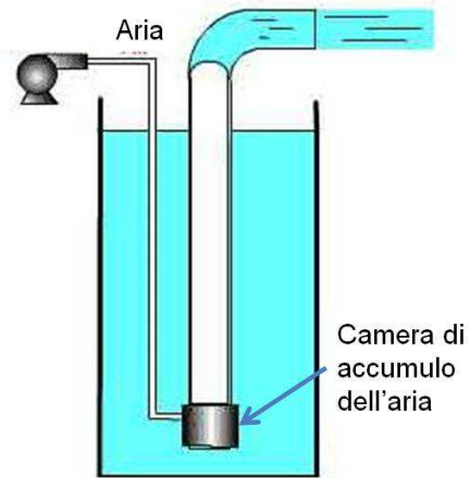
Pompa a Geyser
